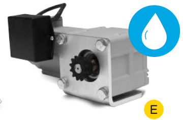
IP67-rated submersible motor.
